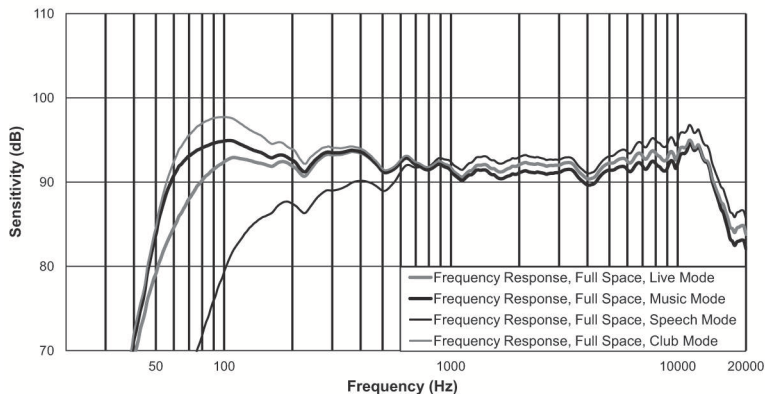
Figure 7.3: Frequency response: 12" powered ZLX models
